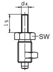
Form G / GN Form GK / GKN
