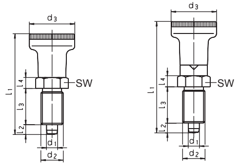
Form A / AN / ANN
